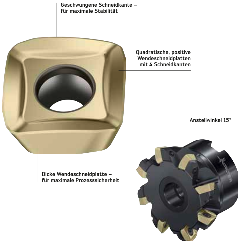
High-Feed-Fräser M4002
